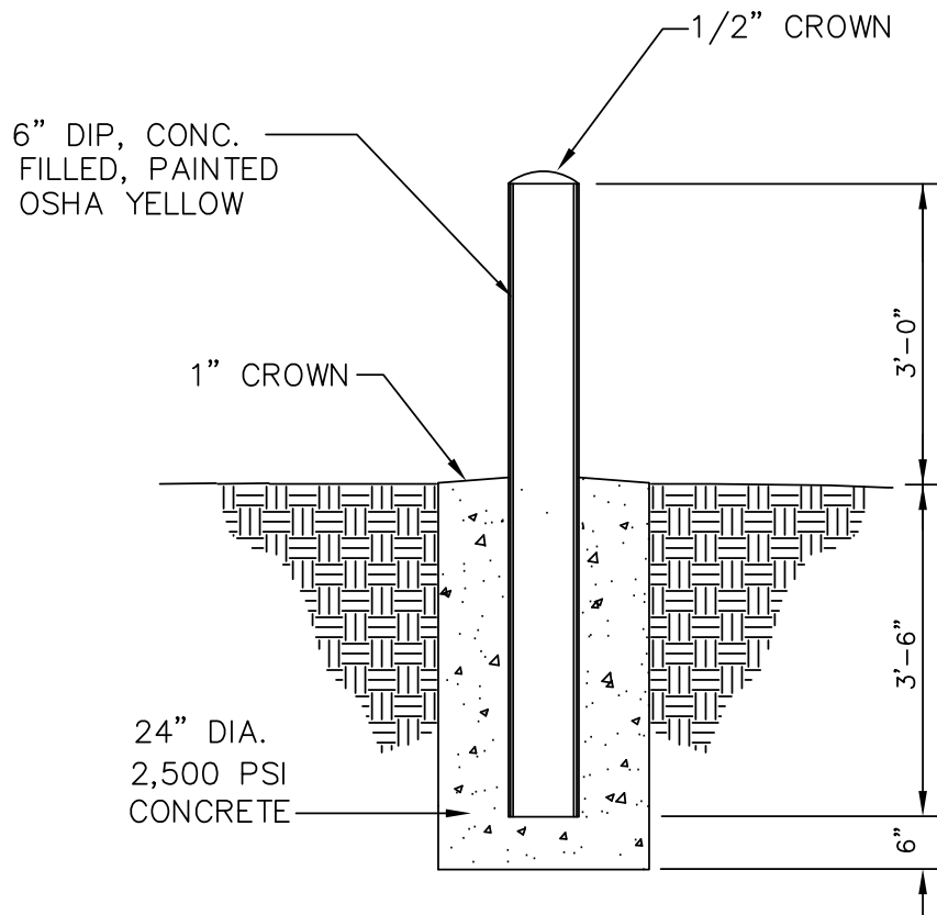
BOLLARD DETAIL
